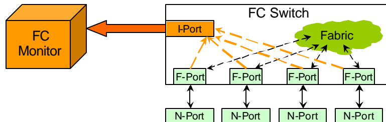
Figure 6. Fibre Channel Switch with non-standard I-Port
