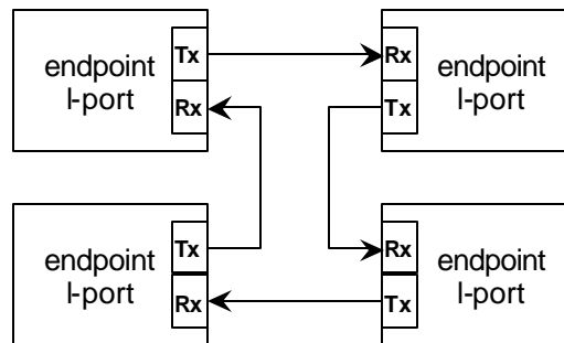
Figure 3. Fibre Channel Arbitrated Loop
