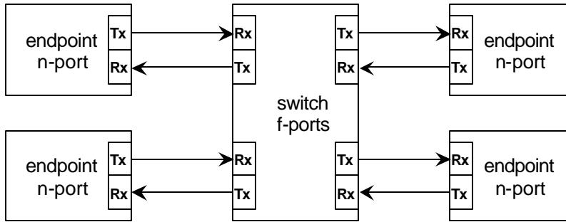
Figure 3. Fibre Channel Switched Fabric
