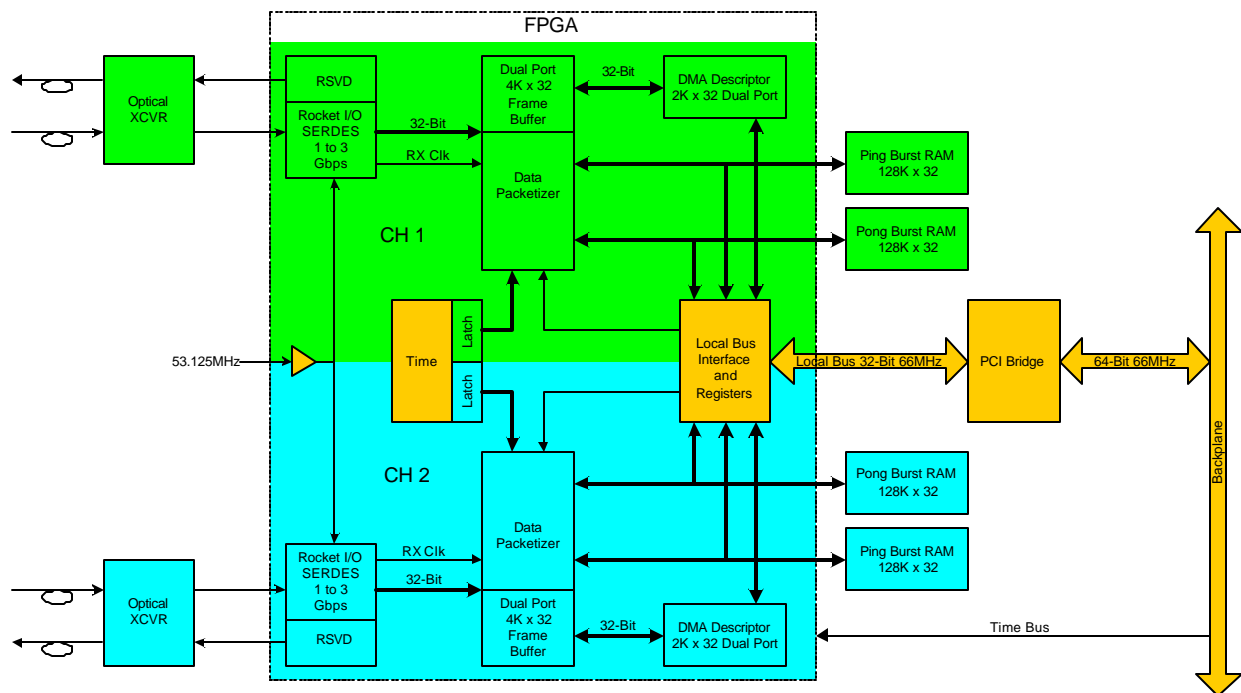
Figure 5. Board and FPGA Block Diagram
