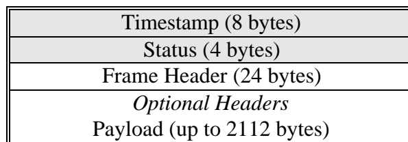
Figure 7. Captured Fibre Channel Frame
