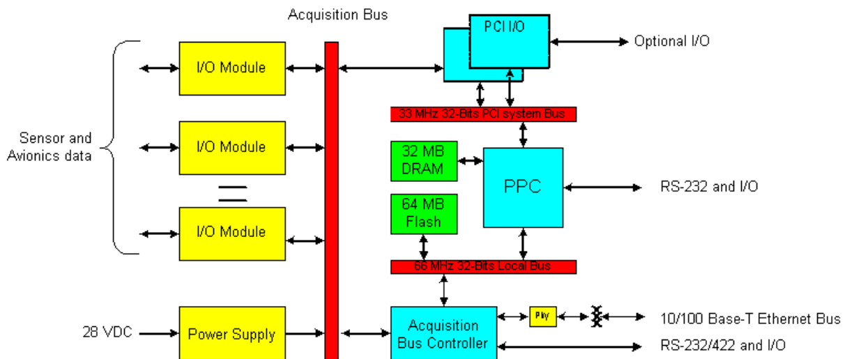
Figure 2. Acquisition Unit Architecture
