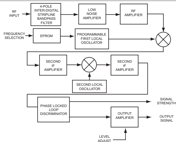
TRS-1110 Series Block Diagram
