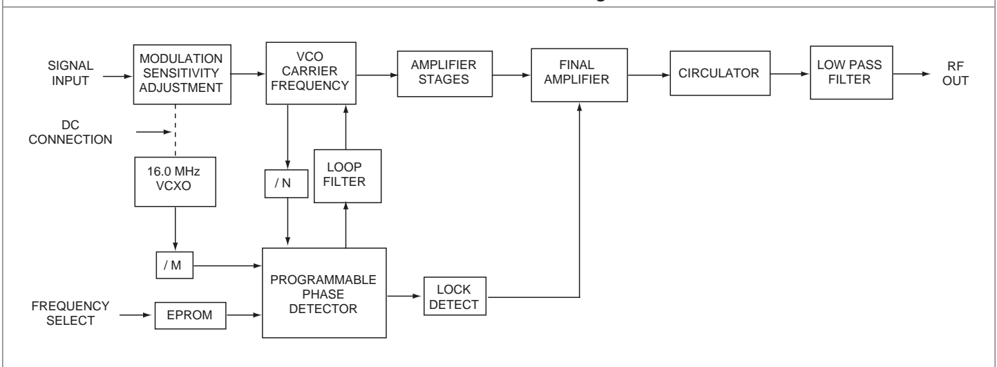
TTS-11000 Series Block Diagram
